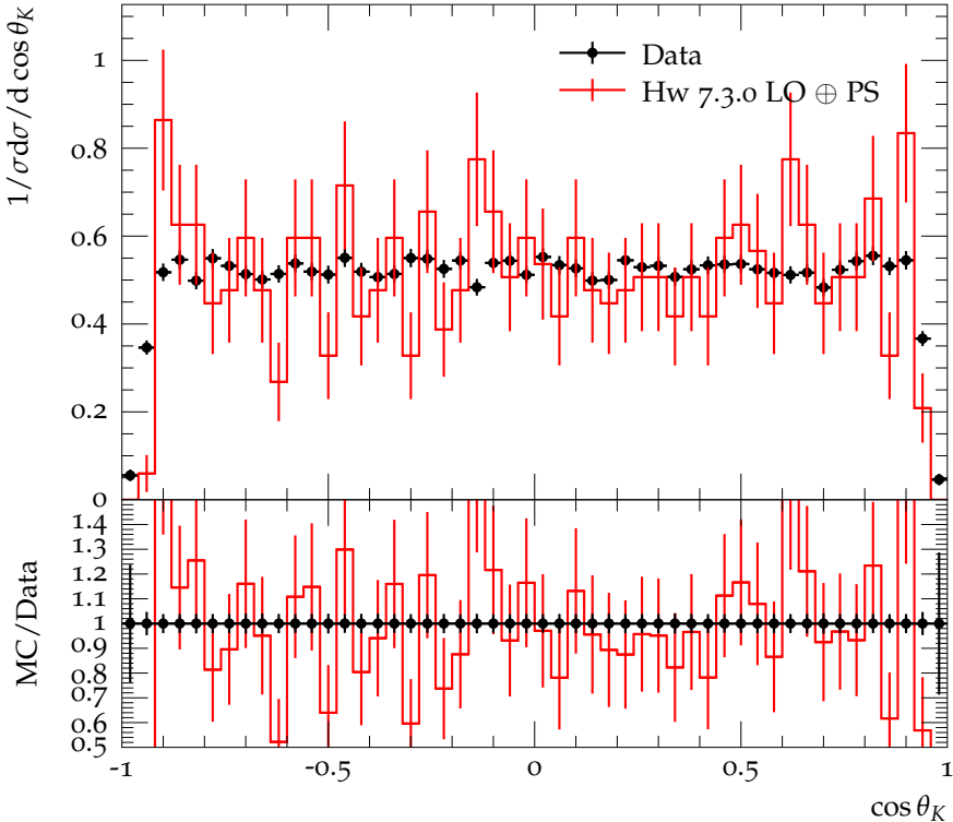
\cos \theta_K distribution for \chi_{c0} production with \chi_{c0} \rightarrow K^+ K^-
