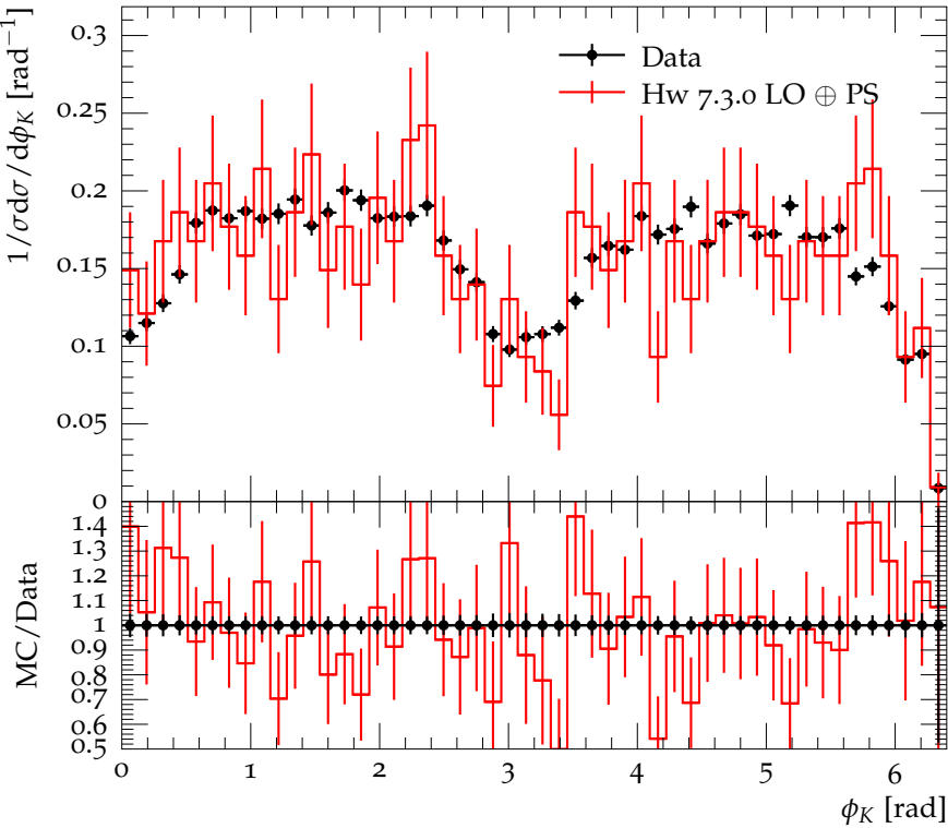
\phi_K distribution for \chi_{c0} production with \chi_{c0} \rightarrow K^+K^-
