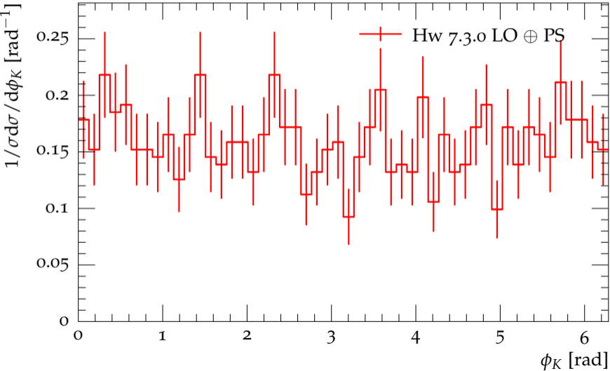
\phi_K distribution for \chi_{c0} production with \chi_{c0} \rightarrow K^+K^- (no cuts)
