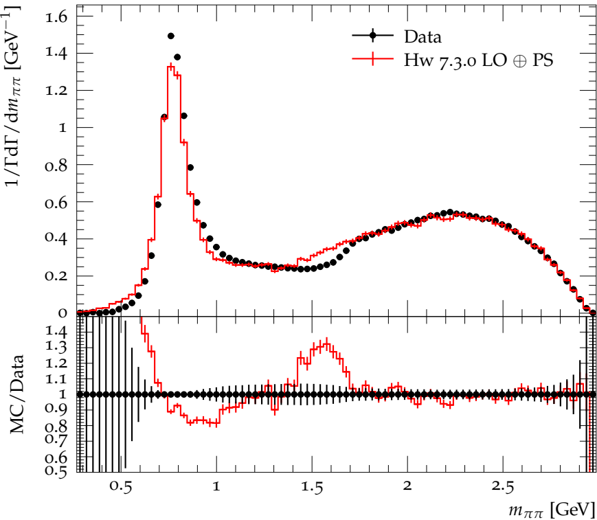
\pi\pi mass distribution in J/\psi \rightarrow \pi^+\pi^-\pi^0
