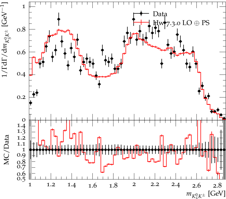
K_S^0 K^\pm mass distribution in \eta_c \rightarrow K_S^0 K^\pm \pi^\mp
