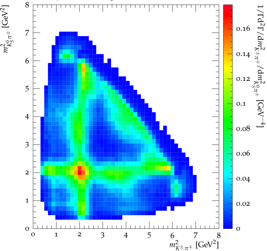
Dalitz plot for \eta_c \rightarrow K_S^0 K^\pm \pi^\mp
