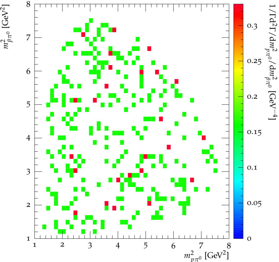
Dalitz plot for \psi(2S) \rightarrow p\bar{p}\pi^0
