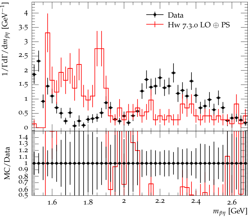
\bar{p}\eta mass distribution in \psi(2S) \rightarrow p\bar{p}\eta
