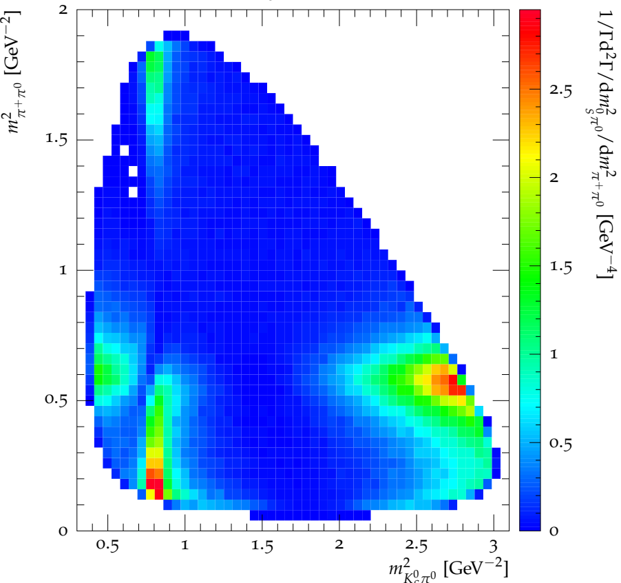
Dalitz plot for D^+ \rightarrow K_S^0 \pi^+ \pi^0
