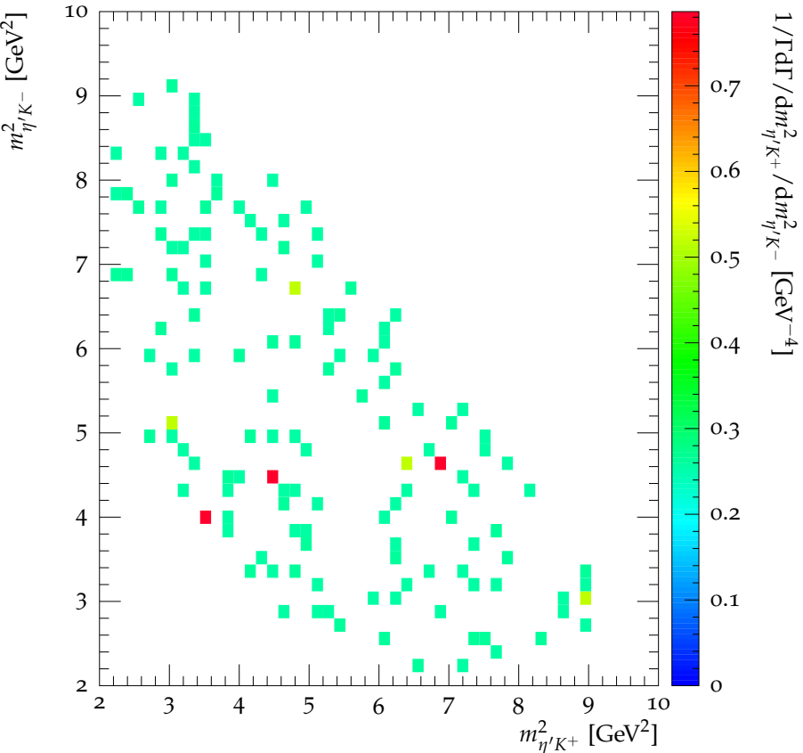
Dalitz plot for \chi_{c1} \rightarrow \eta' K^+ K^-
