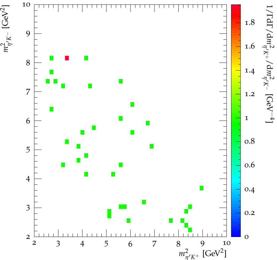
Dalitz plot for \chi_{c2} \rightarrow \eta' K^+ K^-
