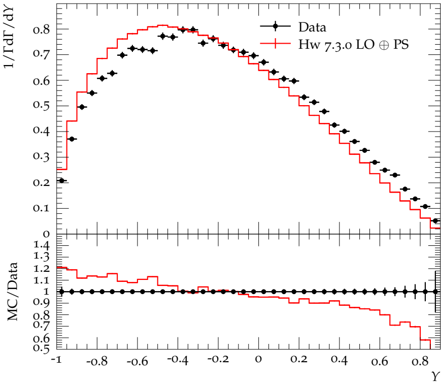
Y distribution for \eta \rightarrow \pi^+ \pi^- \pi^0
