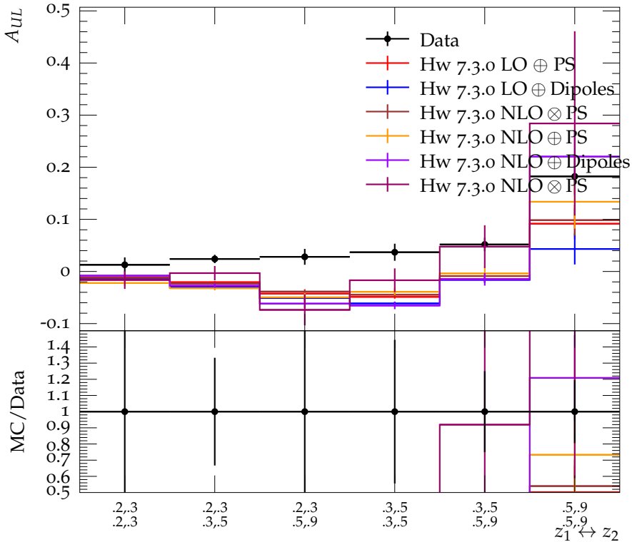
Assymetry for unlike over like sign pion pairs vs z_1, z_2
