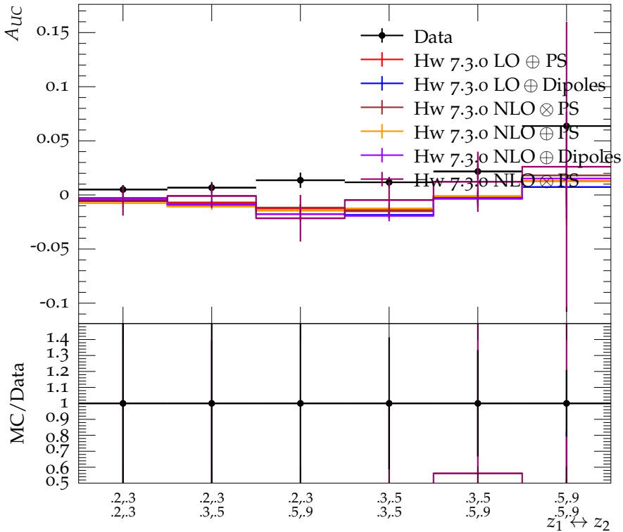
Assymetry for unlike over all pion pairs vs z_1, z_2
