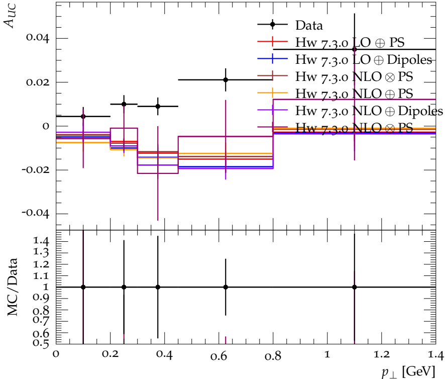
Assymetry for unlike over all pion pairs vs p_{\perp}
