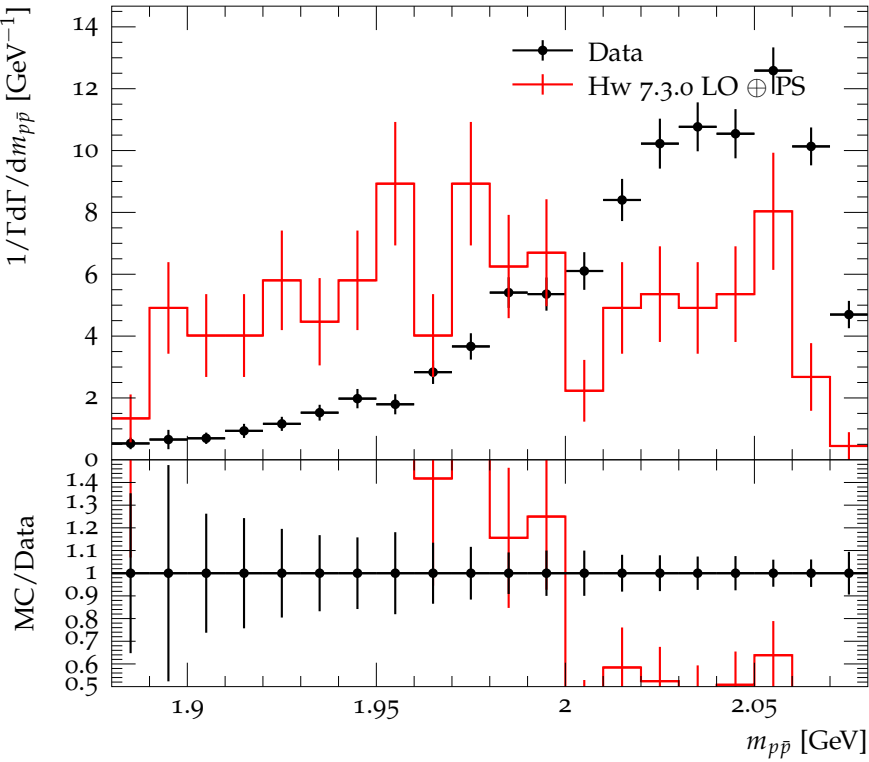
p\bar{p} mass distribution in J/\psi \rightarrow p\bar{p}\phi ( \phi \rightarrow K_S^0 K_L^0 )
