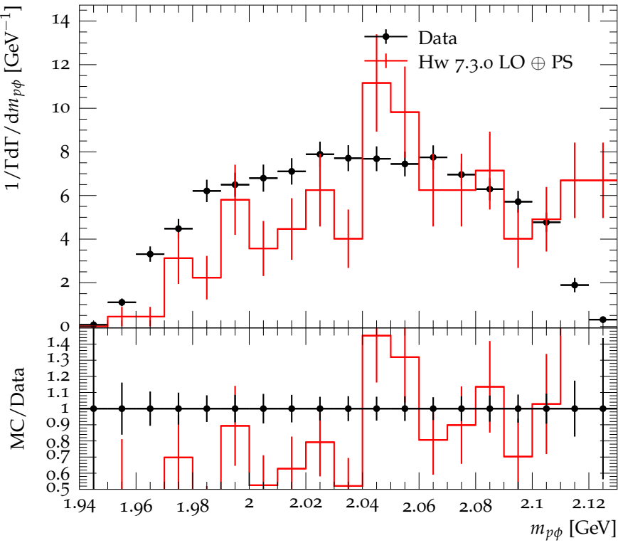
p\phi mass distribution in J/\psi \rightarrow p\bar{p}\phi ( \phi \rightarrow K_S^0 K_L^0 )
