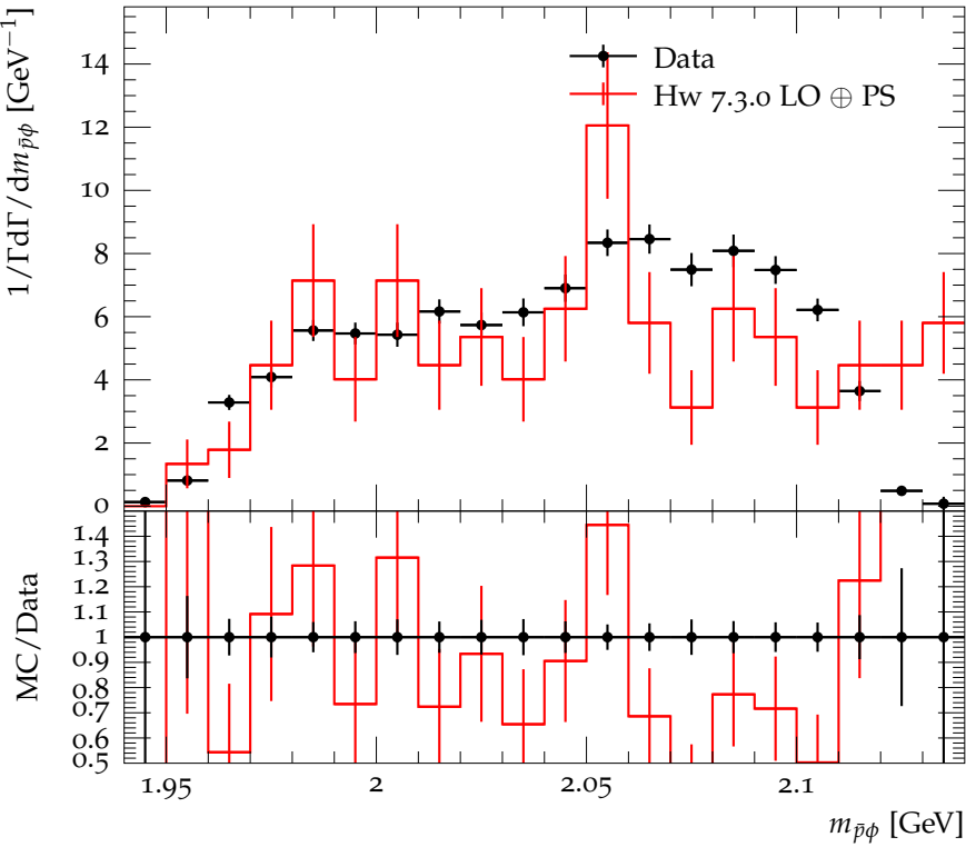
\bar{p}\phi mass distribution in J/\psi \rightarrow p\bar{p}\phi ( \phi \rightarrow K^+K^- )
