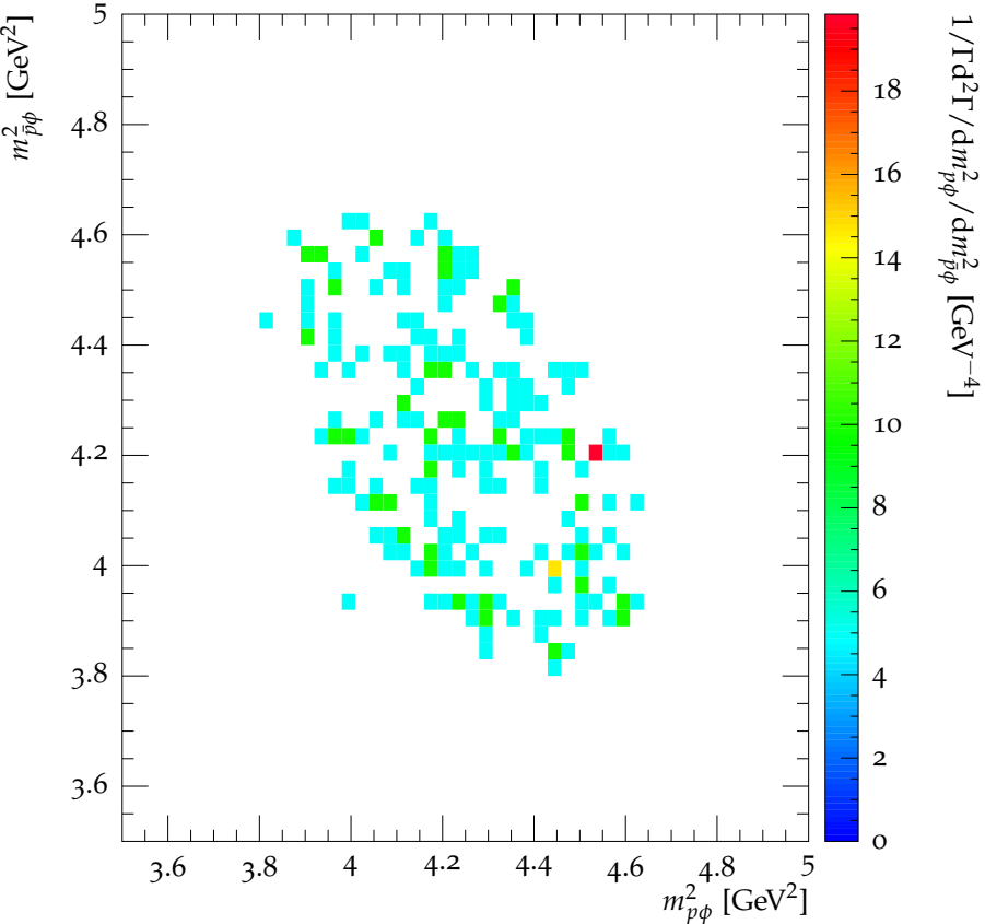
Dalitz plot for J/\psi \rightarrow p\bar{p}\phi
