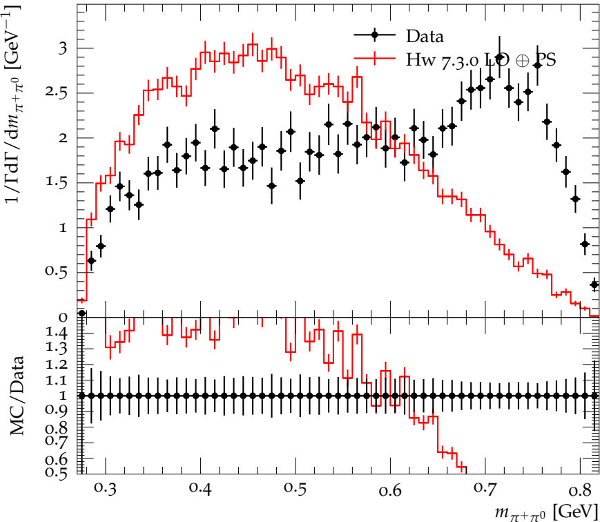
\pi^+\pi^0 mass distribution for \eta' \rightarrow \pi^+\pi^-\pi^0
