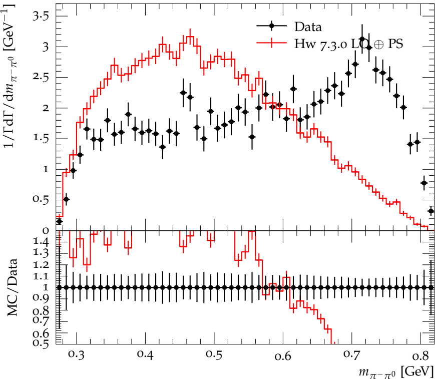
\pi^- \pi^0 mass distribution for \eta' \rightarrow \pi^+ \pi^- \pi^0
