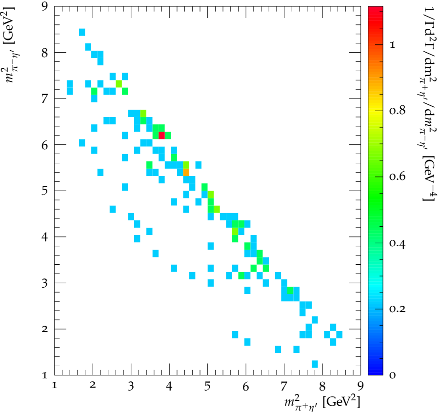
Dalitz plot for J/\psi \rightarrow \pi^+ \pi^- \eta'
