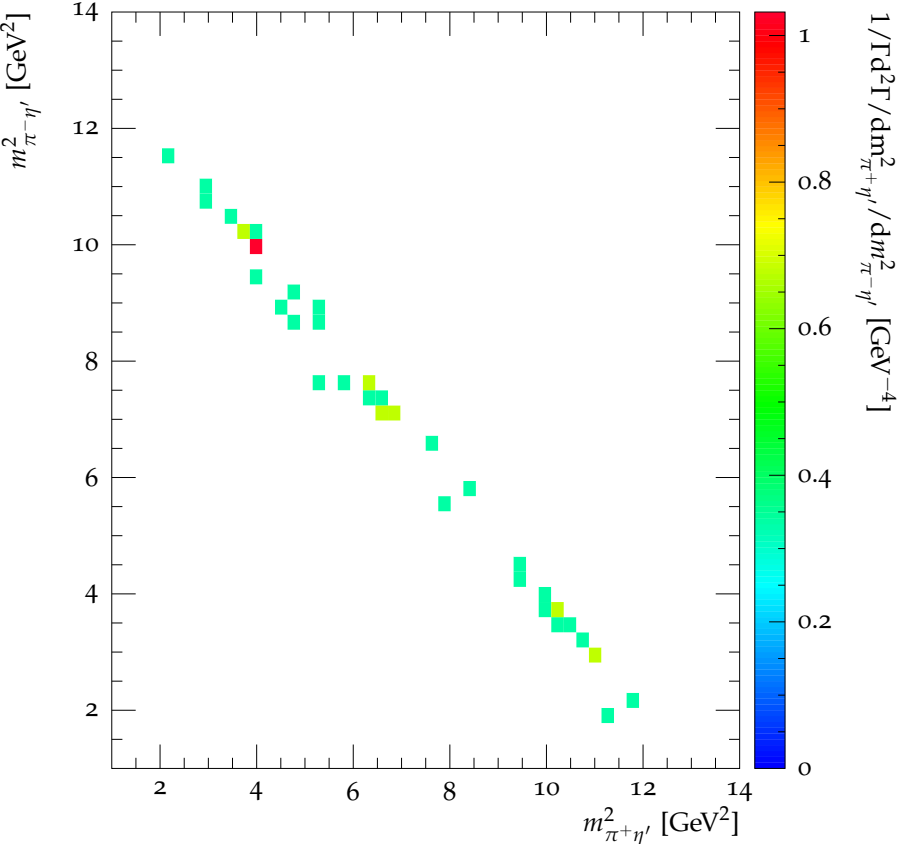
Dalitz plot for \psi(2S) \rightarrow \pi^+ \pi^- \eta'
