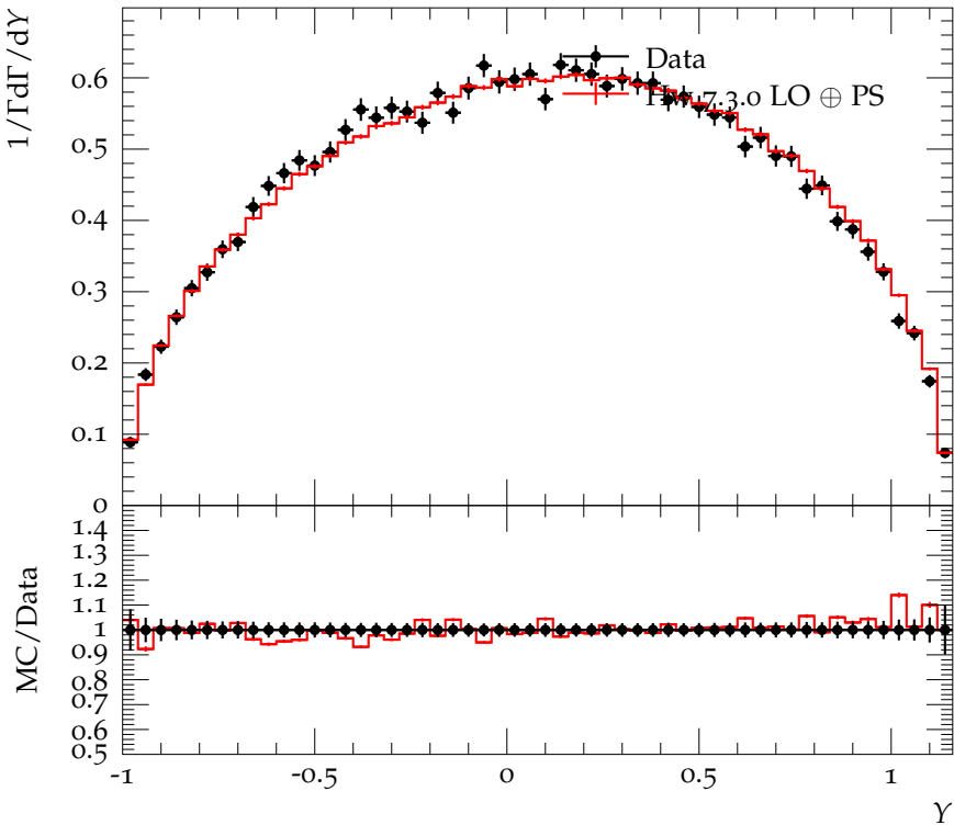
Y distribution for \eta' \rightarrow \eta\pi^0\pi^0
