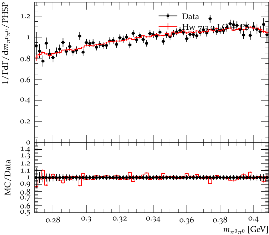
Ratio of m_{\pi^0\pi^0} distribution to phase-space for \eta' \rightarrow \eta\pi^0\pi^0
