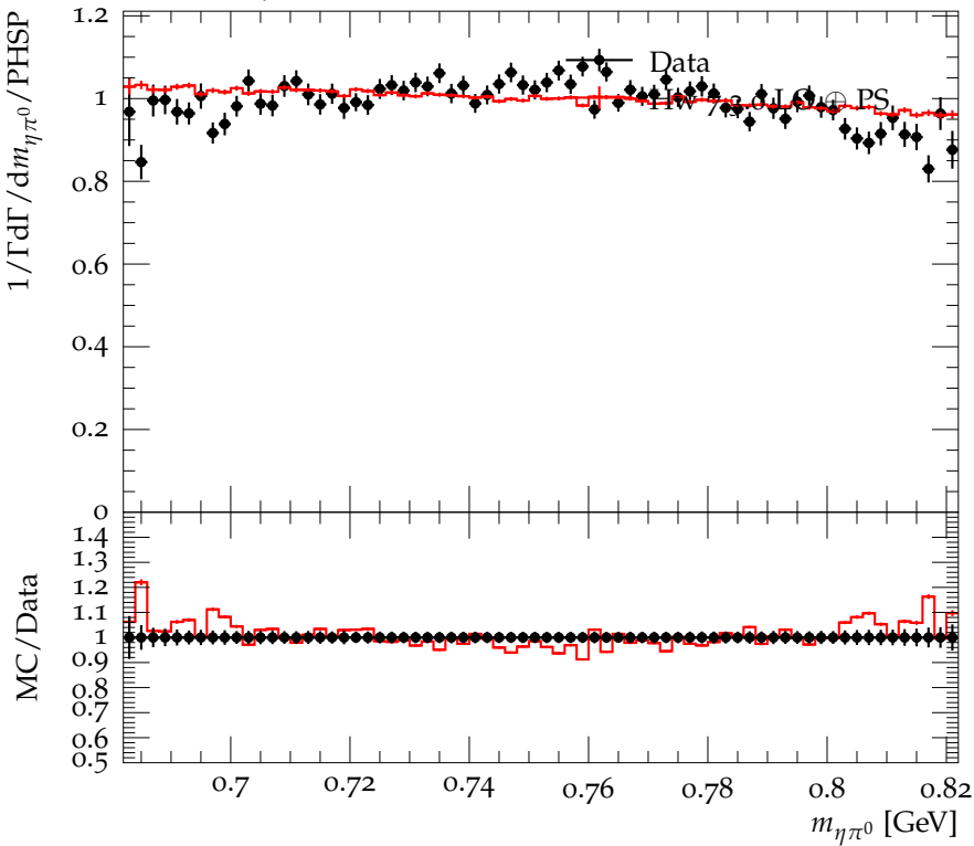
Ratio of m_{\eta\pi^0} distribution to phase-space for \eta' \rightarrow \eta\pi^0\pi^0
