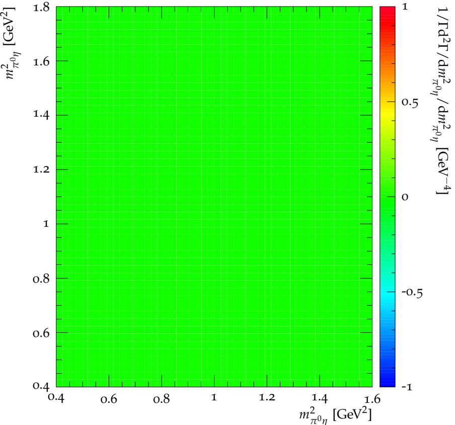
Dalitz plot for D^0 \rightarrow \pi^0 \eta \eta
