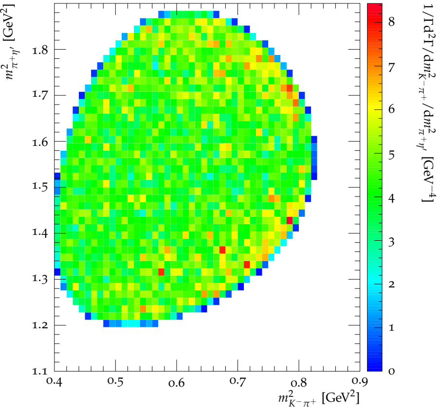
Dalitz plot for D^0 \rightarrow K^- \pi^+ \eta'
