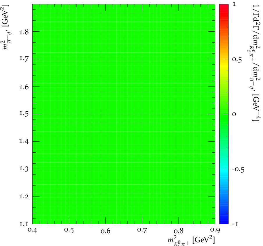
Dalitz plot for D^+ \rightarrow K_S^0 \pi^+ \eta'
