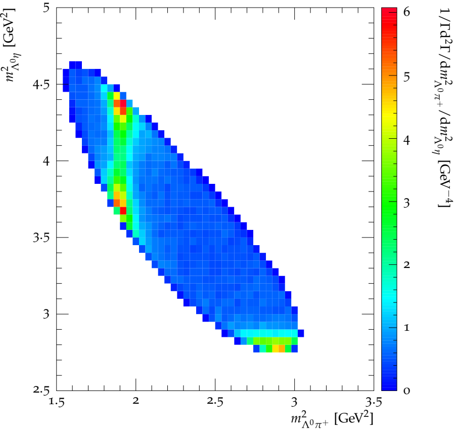
Dalitz plot for \Lambda_c^+ \rightarrow \Lambda^0 \eta \pi^+
