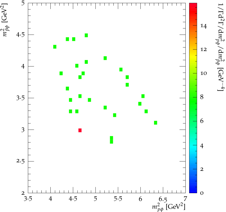
Dalitz plot for J/\psi \rightarrow \phi\eta\eta'
