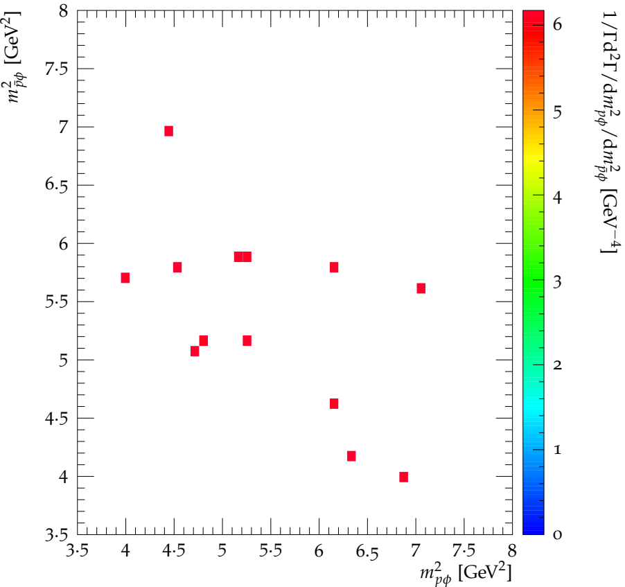
Dalitz plot for \psi(2S) \rightarrow p\bar{p}\phi
