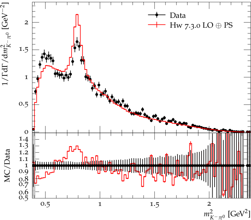
K^- \pi^0 mass distribution in D^0 \rightarrow K^- \pi^+ \pi^0 \pi^0
