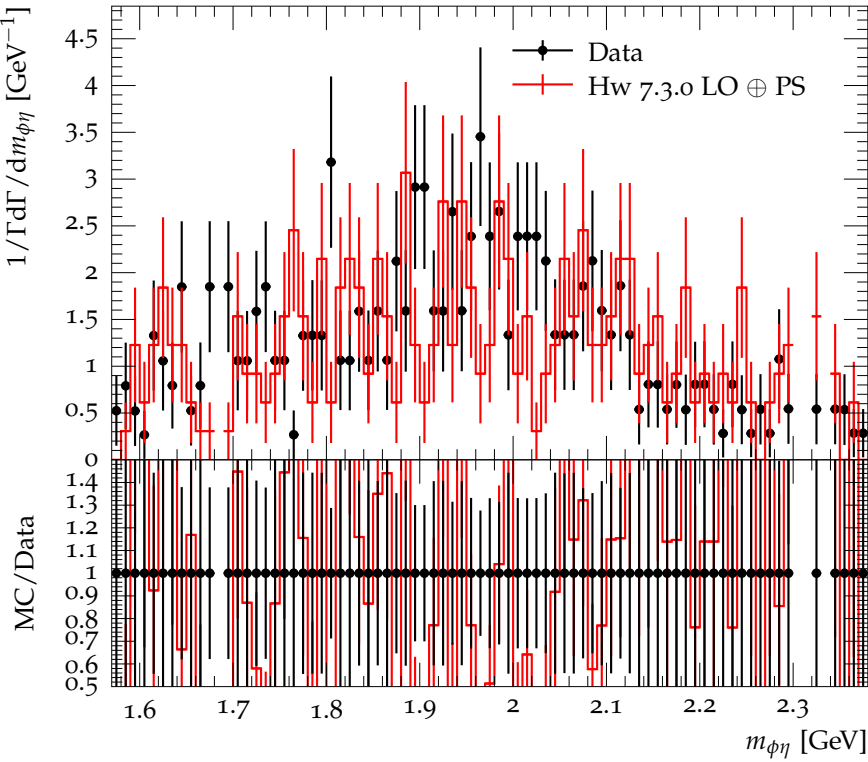
\phi\eta mass distribution in \chi_{c0} \rightarrow \phi\phi\eta
