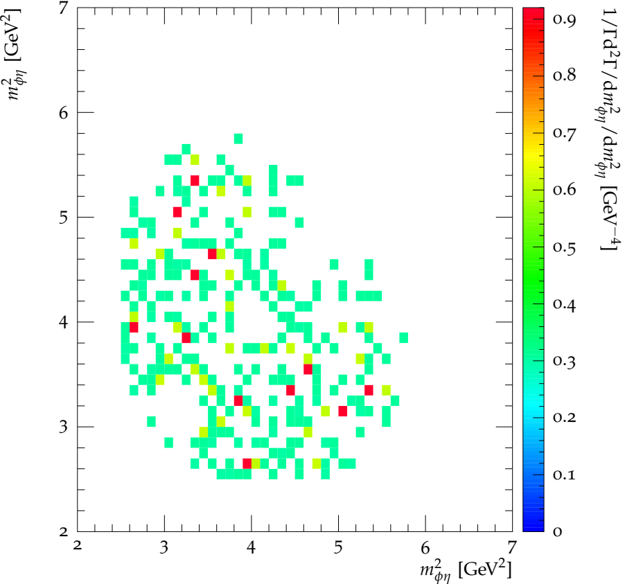
Dalitz plot for \chi_{c0} \rightarrow \phi\phi\eta
