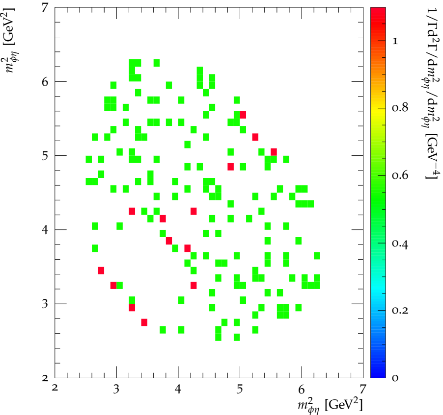
Dalitz plot for \chi_{c2} \rightarrow \phi\phi\eta
