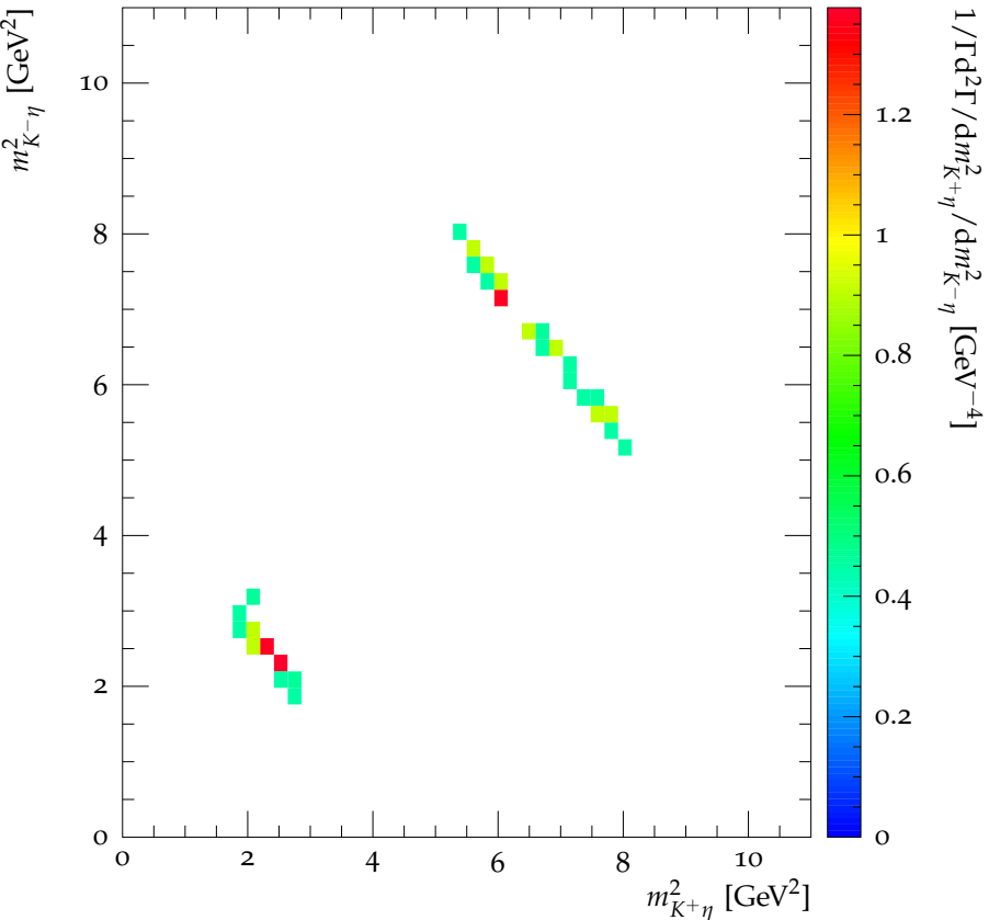
Dalitz plot for \psi(2S) \rightarrow K^+K^-\eta
