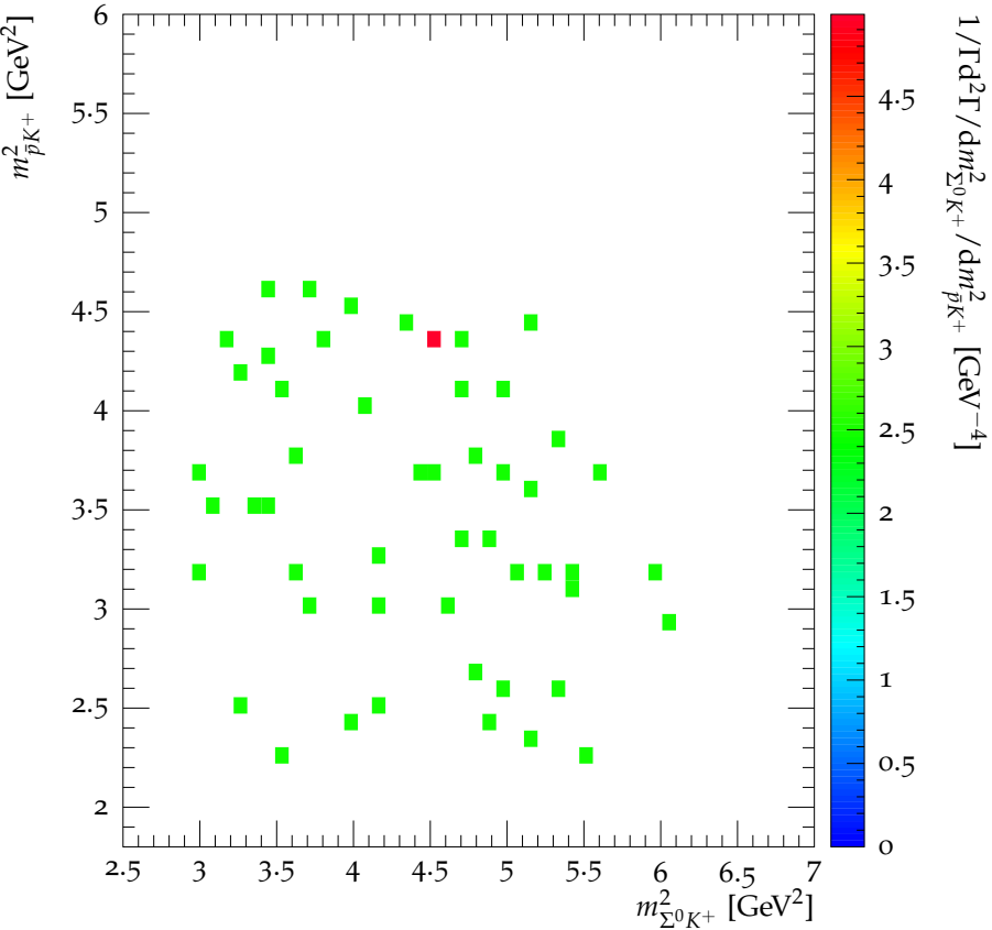
Dalitz plot for \chi_{c0} \rightarrow \Sigma^0 \bar{p}K^+ + \text{c.c.}
