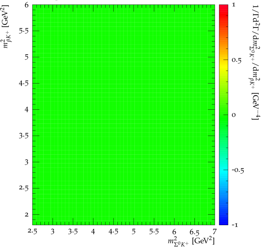
Dalitz plot for \chi_{c1} \rightarrow \Sigma^0 \bar{p}K^+ + \text{c.c.}
