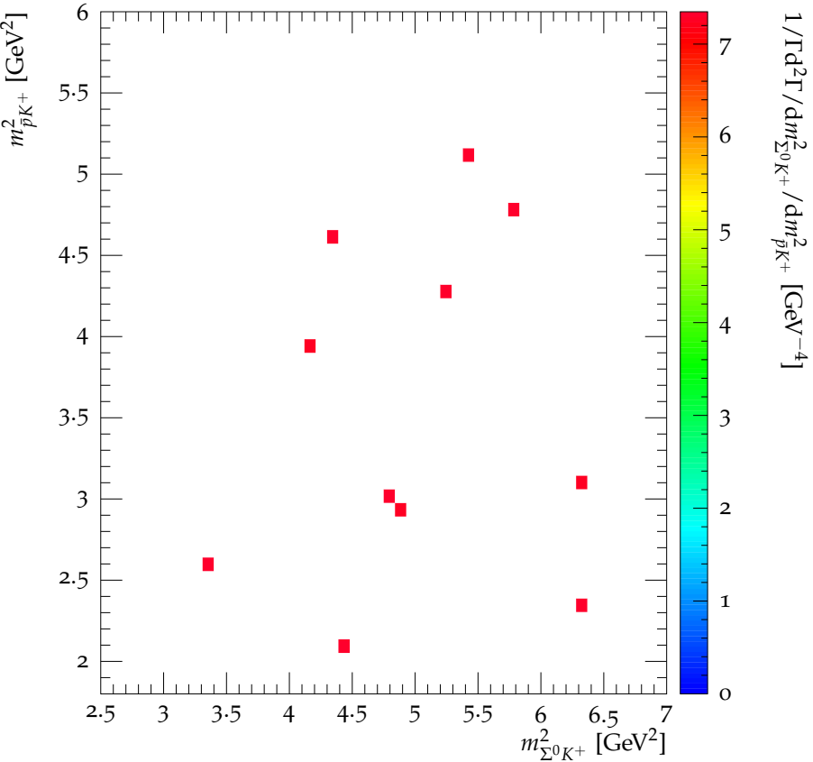
Dalitz plot for \chi_{c2} \rightarrow \Sigma^0 \bar{p}K^+ + \text{c.c.}
