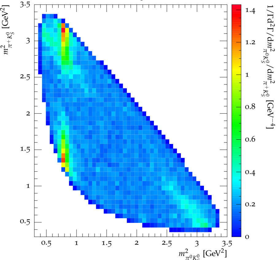
Dalitz plot for D_s^+ \rightarrow \pi^+ \pi^0 K_S^0
