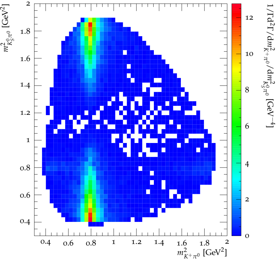
Dalitz plot for D^+ \rightarrow K^+ K_S^0 \pi^0
