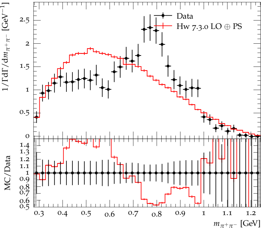
\pi^+\pi^-\ mass distribution in D_s^+ \rightarrow \pi^+\pi^-\pi^-\eta
