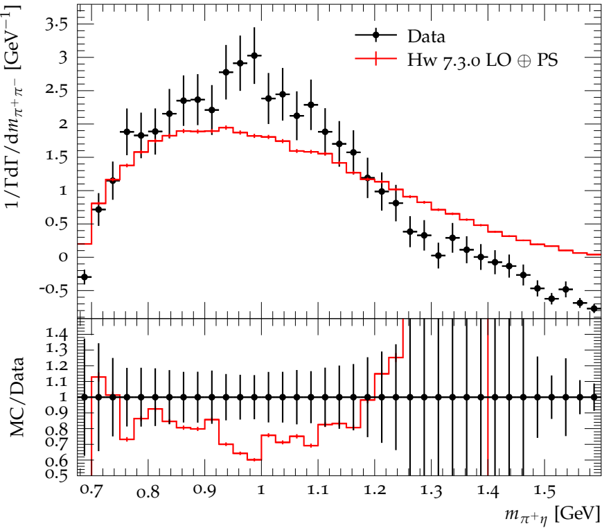
\pi^+ \eta mass distribution in D_s^+ \rightarrow \pi^+ \pi^+ \pi^- \eta
