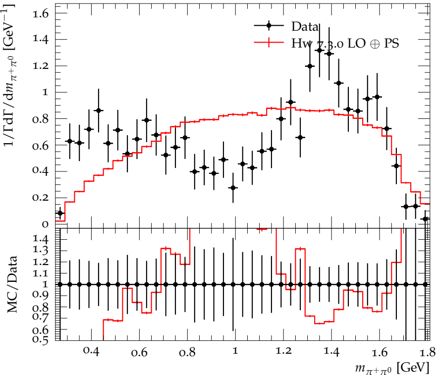
\pi^+\pi^0 mass distribution in D_s^+ \rightarrow \pi^+\pi^0\pi^0
