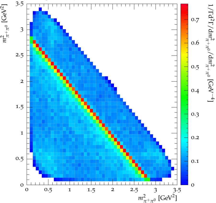
Dalitz plot for D_s^+ \rightarrow \pi^+ \pi^0 \pi^0
