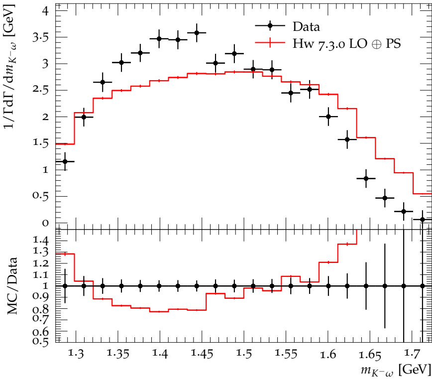
K^- \omega mass distribution in D^0 \rightarrow K^- \pi^+ \omega
