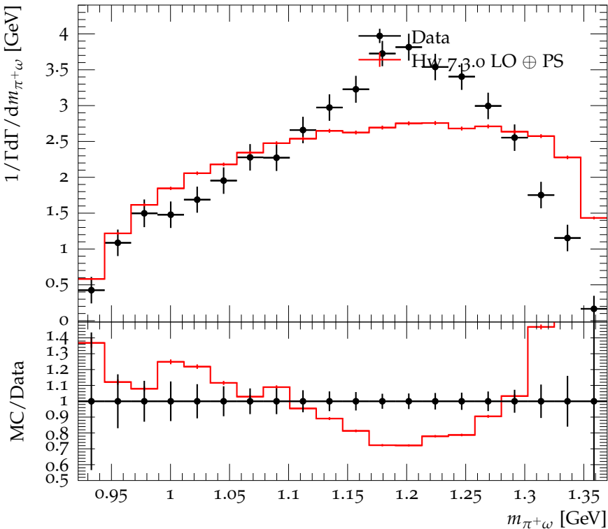
\pi^+\omega mass distribution in D^0 \rightarrow K^-\pi^+\omega
