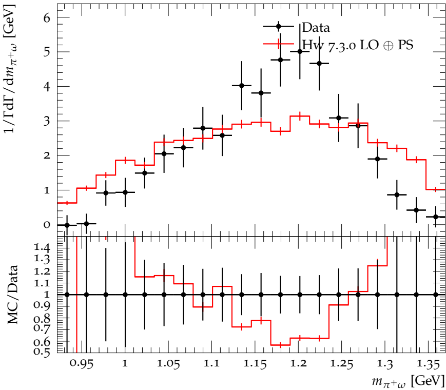
\pi^+\omega mass distribution in D^+ \rightarrow K_S^0\pi^+\omega
