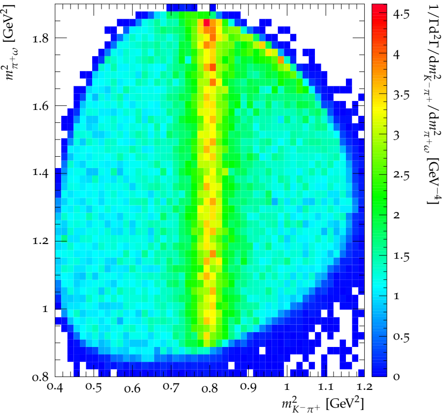
Dalitz plot for D^0 \rightarrow K^- \pi^+ \omega
